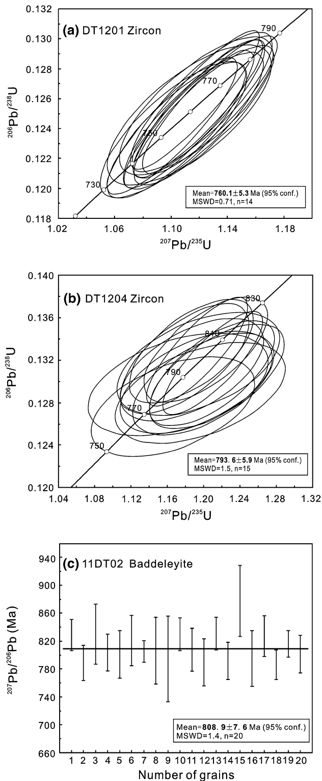
4 SIMS zircon U–Pb concordia diagrams of sample DT1201 and DT1204. SIMS weighted mean ^{207}\text{Pb}/^{206}\text{Pb} ages on 20 baddeleyite grains of sample 11DT02, and the represent 95 % confidence limits of measurements (♣)
